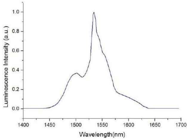
EAT14 Emission
