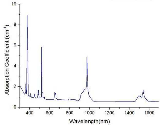
WM4 Absorption
