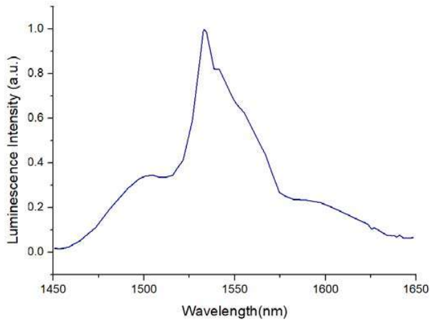
WM4 Emission
