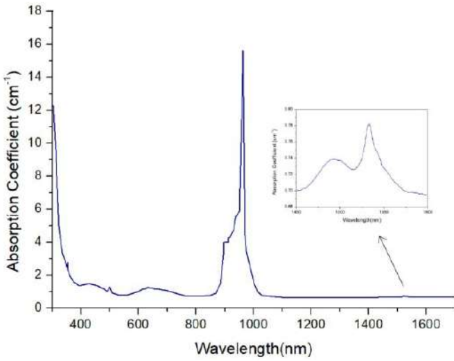
CrE5 Absorption
