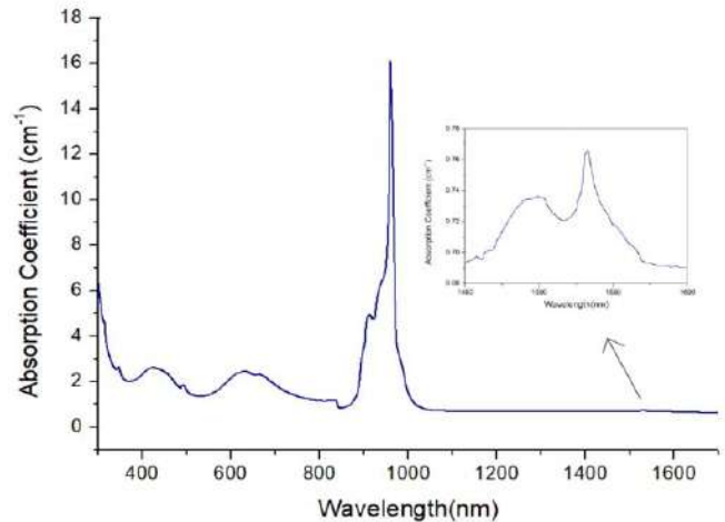
Cr14 Absorption
